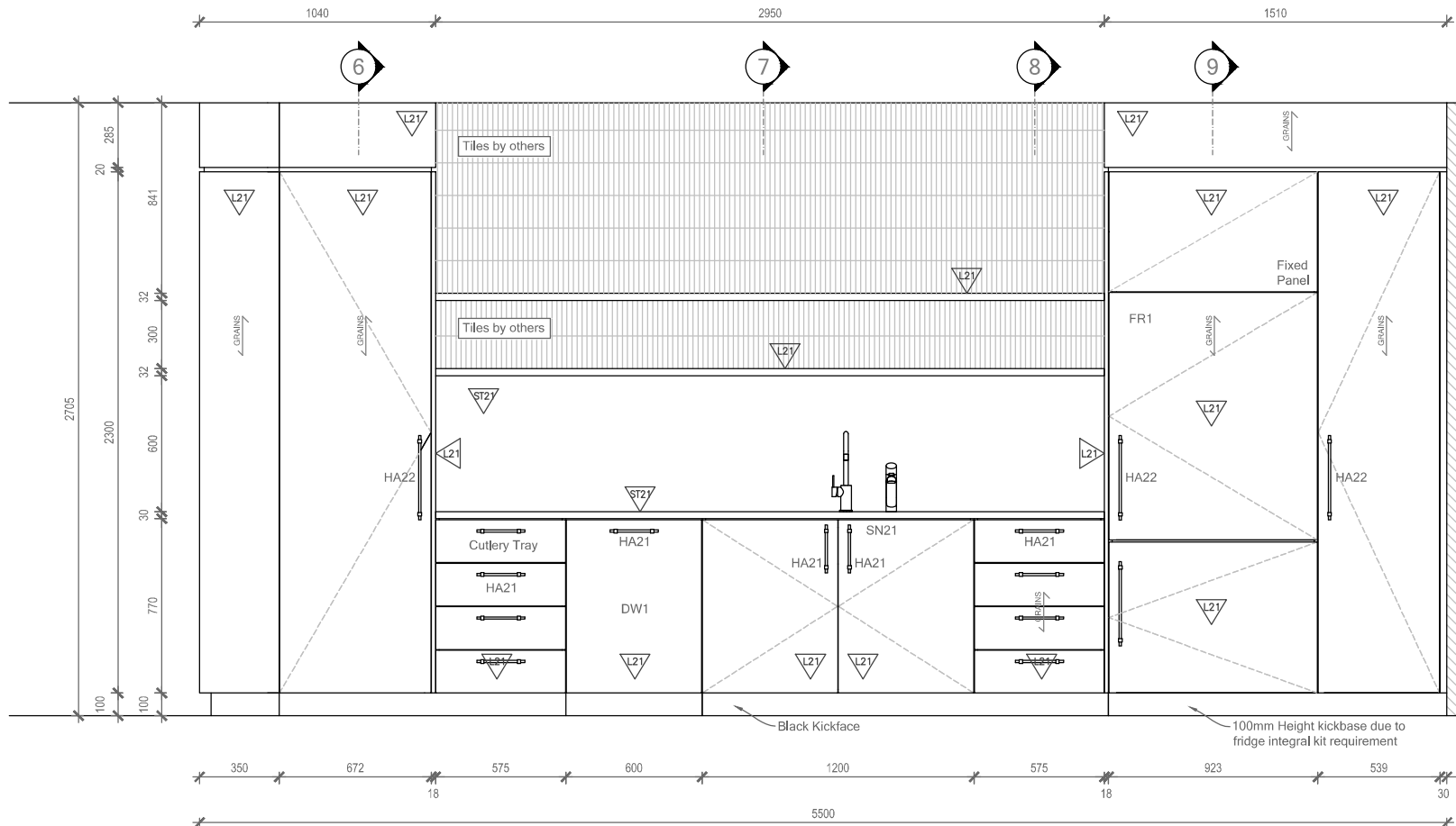
Elevation NTS
