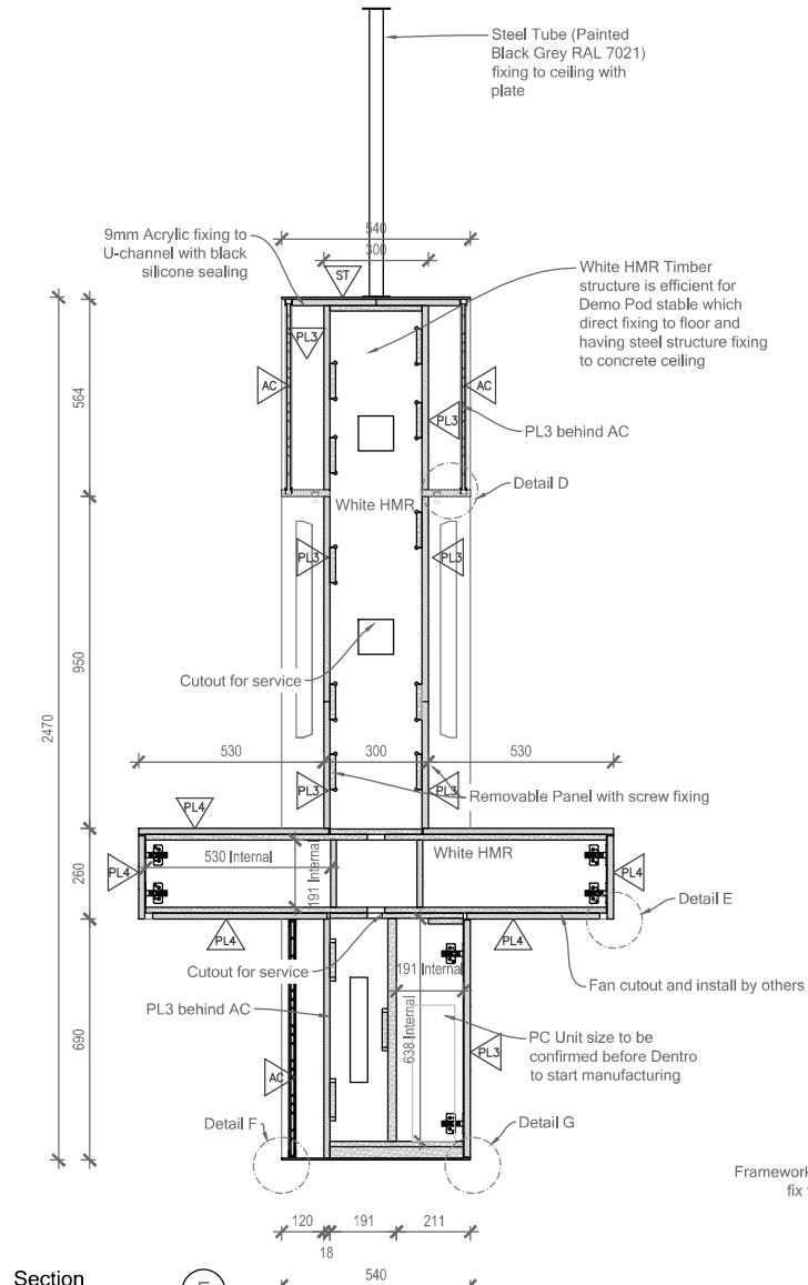
Section NTS
