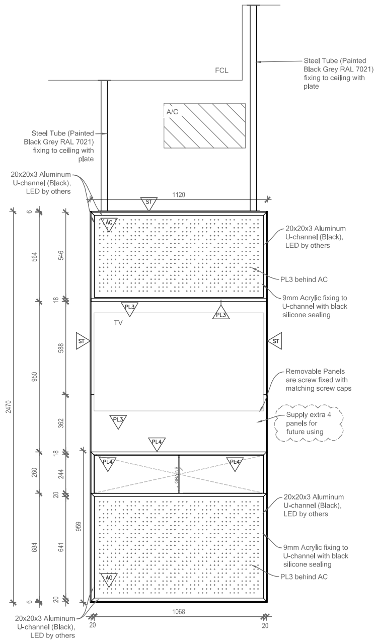
Elevation NTS
