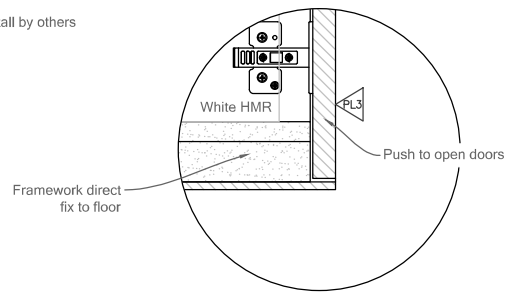
Detail NTS
